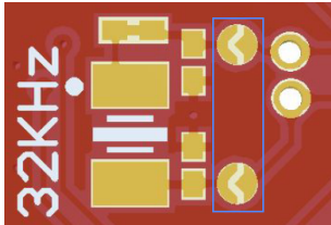
Figure 4-2. Crystal Connection and Cut Straps
